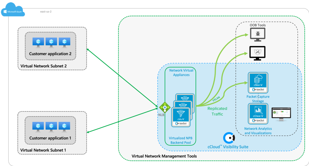
Figure 4 - Microsoft Azure Inter-Subnet example
